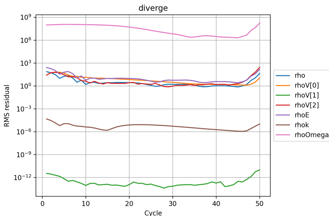
Fig. 5: The typical form of a divergent set of residuals. Rather than decreasing, the values all start increasing significantly from cycle 45 onwards. In this case the NACA0012 case was deliberately set with an unstable explicit CFL number of 6.0.
