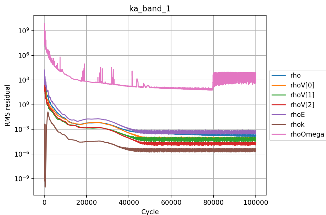
Fig. 6: The convergence of the steady-state explicit solver has achieved an average residual reduction of 5 orders of magnitude and then stalled. The noise in the solution from 40k cycles onwards suggests that either the flow is not fundamentally steady-state or that multigrid is adding an error to the solution. The user must determine whether the level of convergence is sufficient for their purposes and if not whether to run an unsteady simulation or degrade the spatial accuracy.
