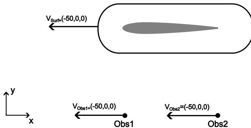
Fig. 4: FWH simulation of an airfoil, with quiescent medium co-ordinate transformation applied
