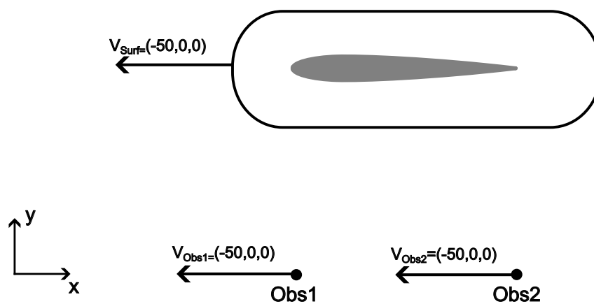
Fig. 1.5: FWH simulation of an aerofoil, with quiescent medium co-ordinate transformation applied
