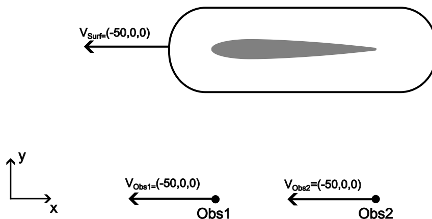
Fig. 1.5: FWH simulation of an aerofoil, with quiescent medium co-ordinate transformation applied
